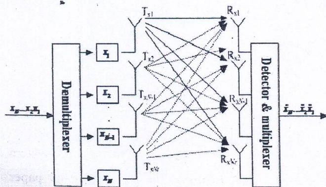
Fig. 1. SDM system model
