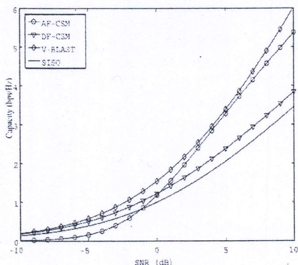
Fig. 7. The capacity results of 2 x 2 AF-CSM system compared with other systems.
