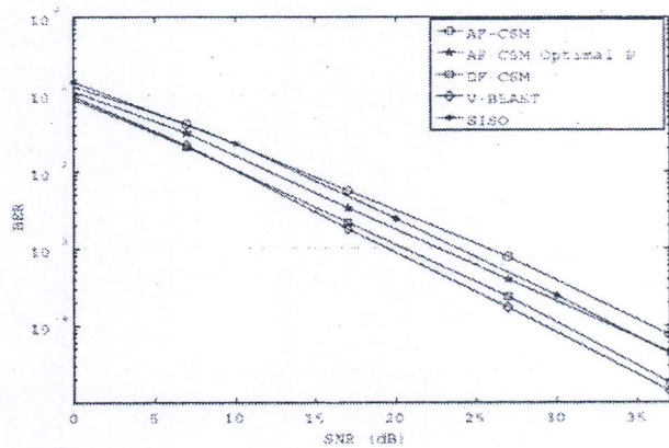
Fig. 4. BER Comparison of AF-CSM with other systems
