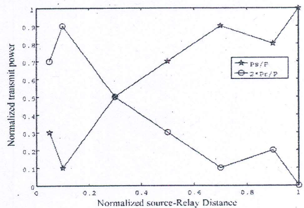
Fig. 7. Simulation results of optimal power allocation, SNR = 40dB.
