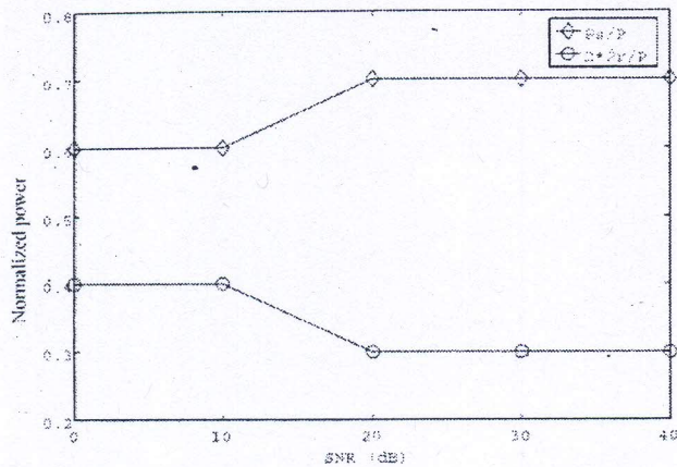
Fig. 5. Power distribution of AF-CSM system.
