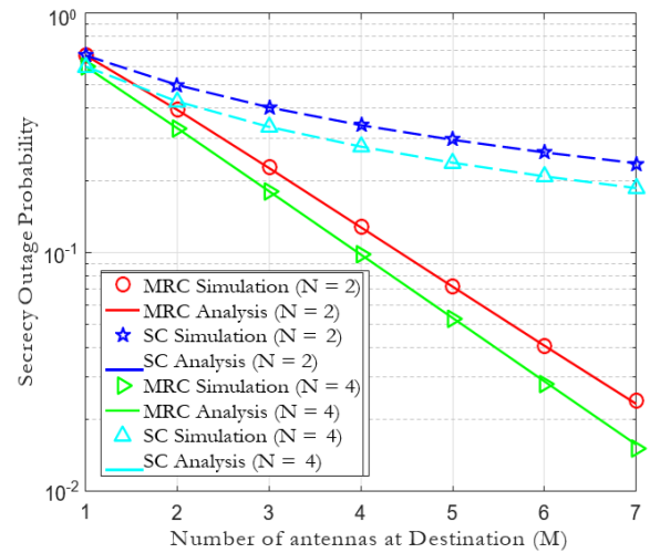
Figure 3. Secrecy outage probability (SOP) vs. number of antennas at the destination ( M ) for different scenarios of MRC and SC.
