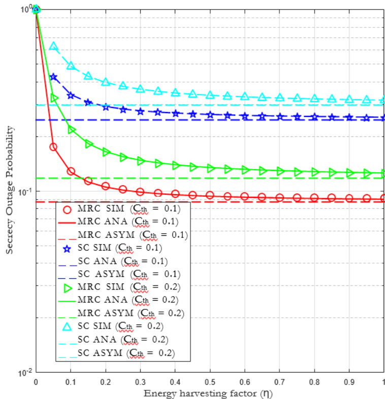
Figure 4. Impact of \eta and C_{th} on secrecy outage probability (SOP) for various MRC and SC configurations.
