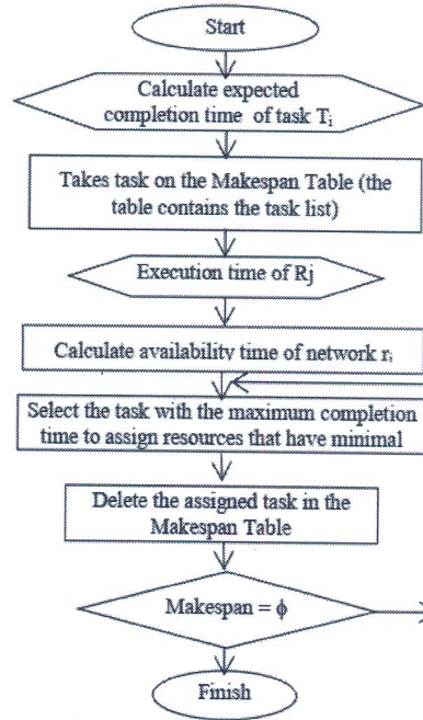
Figure 6. Max-Min Scheduling algorithm schema
