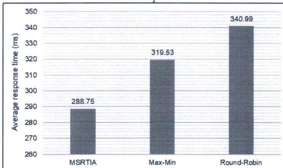
Figure 13. Experimental result after 4 times counted on average
