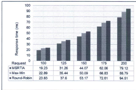
Figure 10. Experimental result on 4 virtual machines with 200 requests
