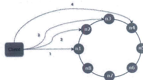
Figure 3. Round-Robin algorithm
