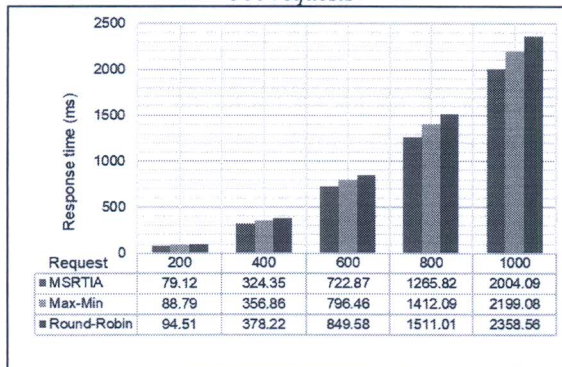
Figure 12. Experimental result on 4 virtual machines with 1000 requests
