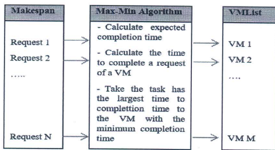
Figure 5. Max-Min Scheduling algorithm operation
