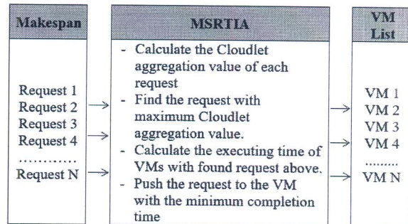
Figure 7. MSRTIA based on Cloudlet aggregation value
