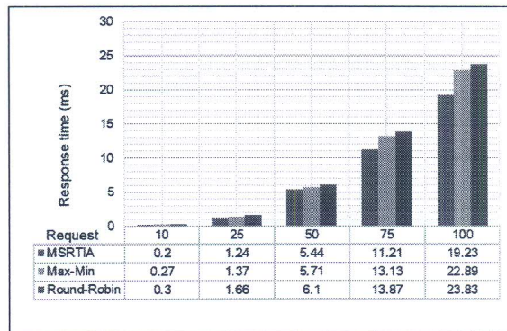
Figure 9. Experimental result on 4 virtual machines with 100 requests
