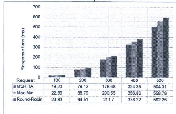
Figure 11. Experimental result on 4 virtual machines with 500 requests
