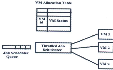
Figure 4. Throttled algorithm
