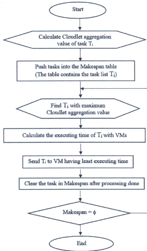
Figure 8. MSRTIA schema
